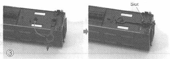
Insert the hook on the assembled coupler to the slot under the floor part, and turn the coupler as on the photo. Then reassemble the truck.
