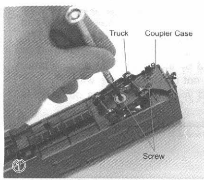
Detach Coupler Cases and Trucks from the floor part by removing each part's screw.
