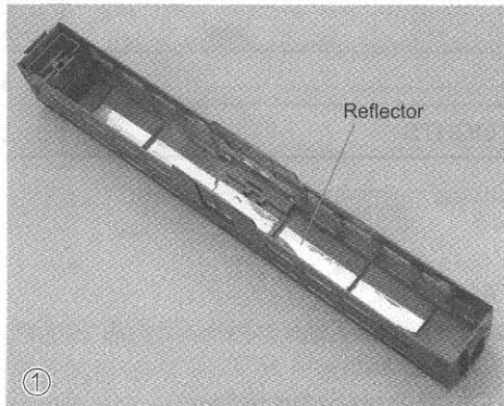
After disassembling the bodyshell and floor part, install the Reflector to the ceiling.
