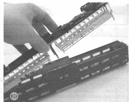
To avoid the light unit's dropping, put the bodyshell upside down when reassembling.
