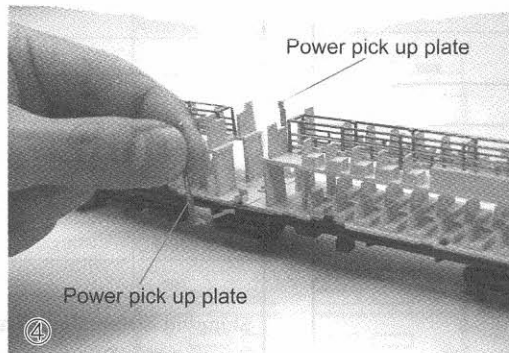
Install the two Power pick up plates as on the photo.
